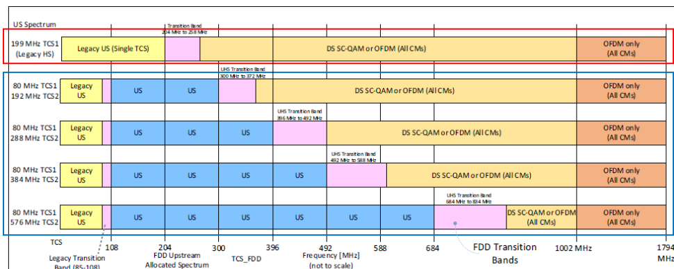
DOCSIS 3.1 High-Split Mode
